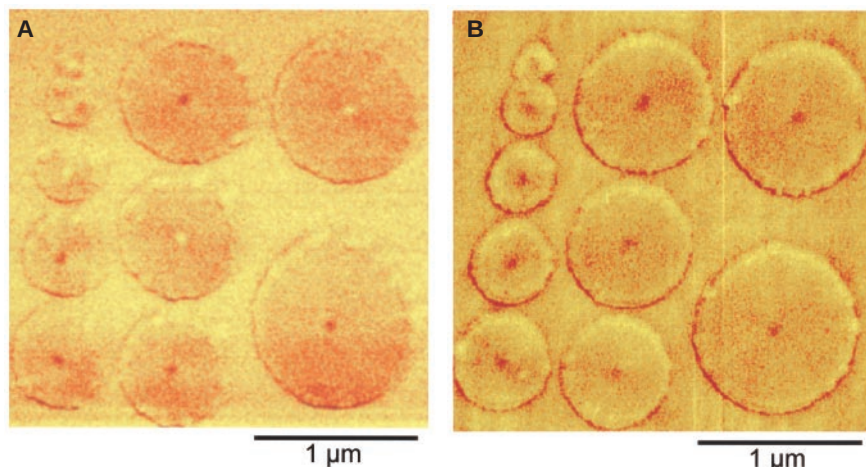
Fig. 3. MFM image of an ensemble of 50-nm-thick permalloy dots with diameters varying from 0.1 to 1 \mu\text{m} after applying an external field of 1.5 T along an in-plane direction (A) and parallel to the plane normal (B).
