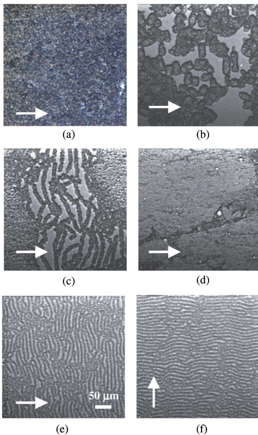
FIG. 4 (color online). Microphotographs of emulsions with \phi = 0.58 under simple shear for gap thicknesses of (a)–(d) 20 \mu\text{m} and (e),(f) 12 \mu\text{m} . Arrows indicate the direction of shear. The reference scale for all frames is inserted in frame (e).
