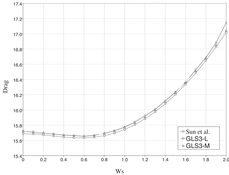
Fig. 1. Flow past a circular cylinder: drag as a function of Weissenberg number for GLS3 versus Sun et al. [8].
