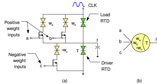
Fig. 1. A monostable-bistable logic element and its equivalent LTG.
