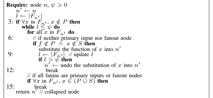
Fig. 4. The node collapsing algorithm.
