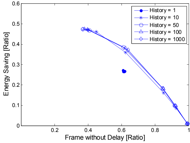
(a) NS-2
