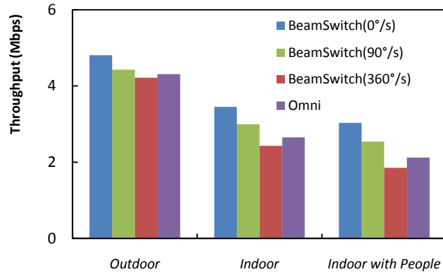
Figure 9: FTP throughput
