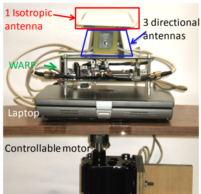
Figure 4: based BeamSwitch prototype on the rotatable platform for experimentation
