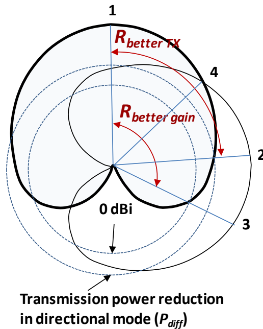
Figure 3: Radiation patterns of a beam (in grey), its neighbor, and the omni antenna with 0dBi gain
