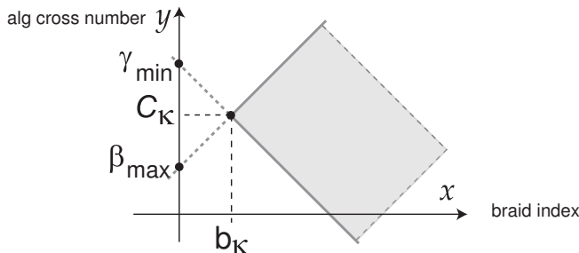
Figure 11: The region of braid representatives of \mathcal{K}
