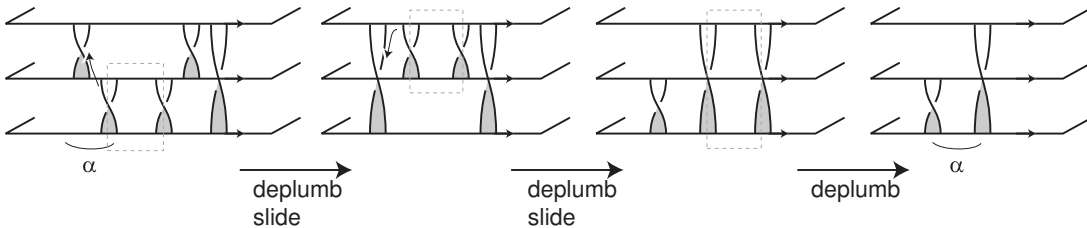
Figure 8: \alpha^2 \longrightarrow \alpha .
