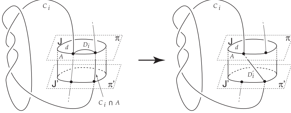
Figure 13: Construction of K_i from \hat{K}_i
