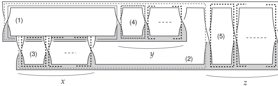
Figure 10: The Bennequin surface F of C_{x,y,z} = \bar{2}1^x 2^y 3^z and a basis for H_1(F)
