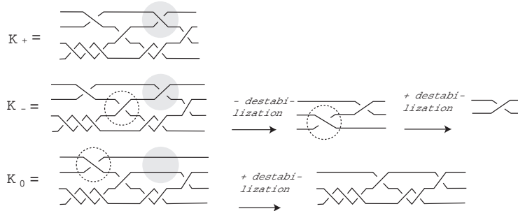
Figure 2: Knot 9_{42} satisfies the conditions of Theorem 2.2
