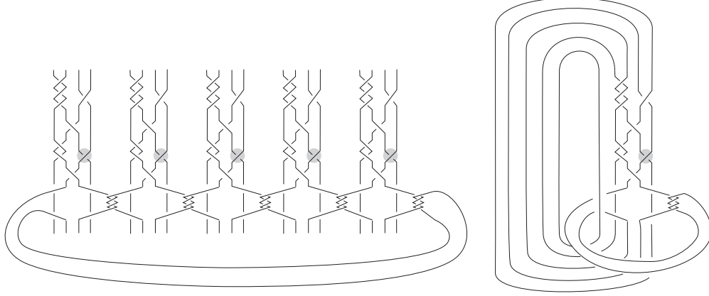
Figure 3: Prime link \mathcal{A}^5(9_{42}) and 2-component link \mathcal{A} .
