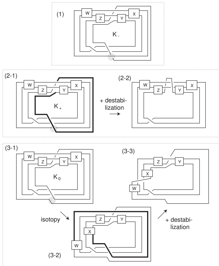
Figure 5: BM-diagram satisfies the sufficient condition
