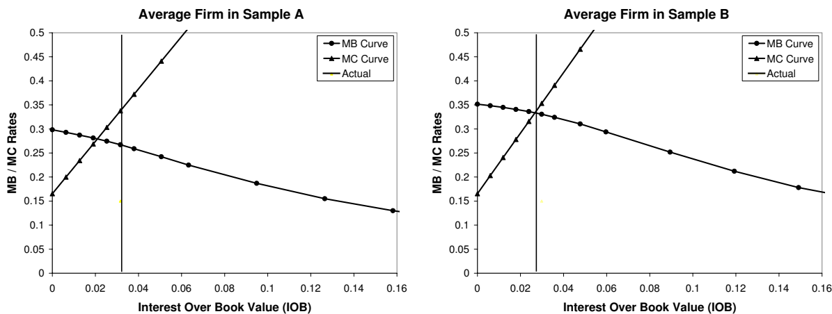
Figure 4: The average (representative) firm in Samples A and B. The marginal benefit curves are based on the average marginal tax benefit and interest over book values for each representative sample. The marginal cost curves are obtained using equation 12 and sample means of the standardized cost control variables.
