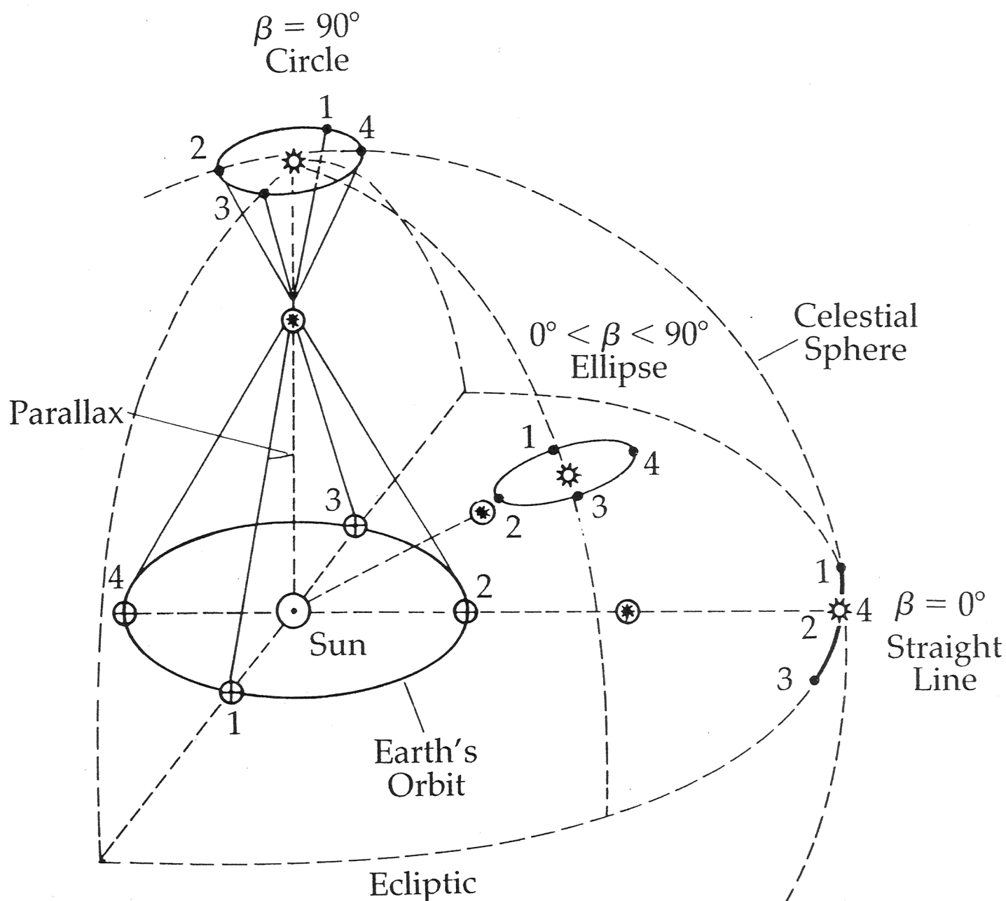
FIGURE 3–14 Parallactic orbits. The Earth's orbital change results in a periodic motion of stellar positions. Note that these are 90^\circ out of phase with respect to the aberration orbits (Figure 3–12) and their angular size depends on the distance to the star. Their shapes depend on their celestial latitude, \beta .
