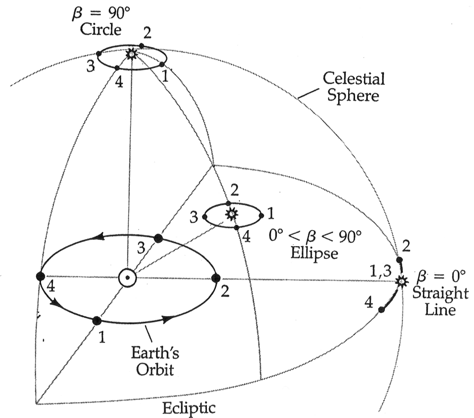
FIGURE 3-12 Apparent stellar orbits resulting from the aberration of starlight. The Earth is shown at four positions in orbit around the Sun (1 to 4). The apparent paths traced out by stars because of the change in the direction of aberration during a year are shown for stars directly above the orbital plane (ecliptic pole), in the plane (the ecliptic), and at an intermediate position on the celestial sphere. The sizes of the apparent orbits are independent of the distances to the stars.
