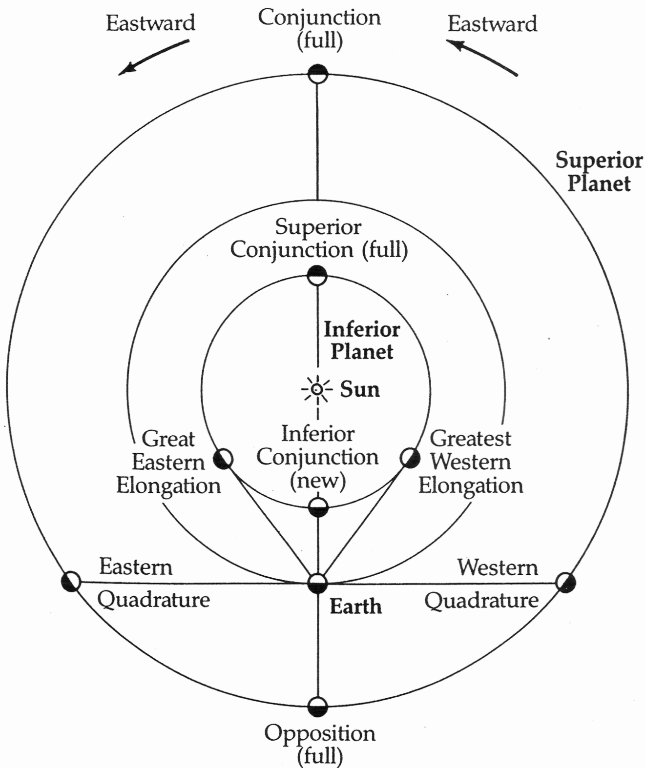
FIGURE 1-2 Heliocentric planetary configurations. Arrows indicate the direction of orbital motion as well as the rotational direction of the Earth. The phases of the planets' illumination are also shown.
