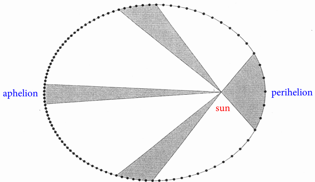
Figure 2.2 Kepler's second law states that the area swept out by a line between a planet and the focus of an ellipse is always the same for a given time interval, regardless of the planet's position in its orbit. The dots are evenly spaced in time.
